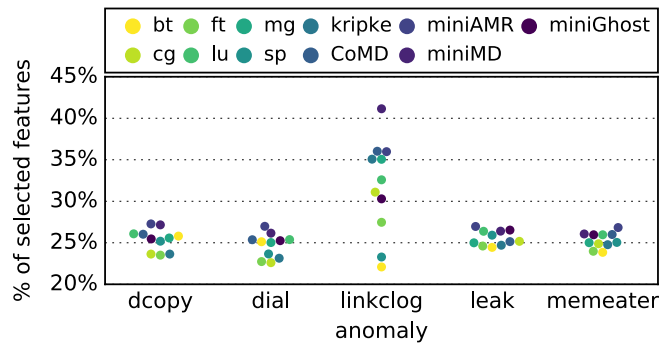
Fig. 4. The percentage of features selected by our feature selection method (Sec. 3.2) for different application-anomaly pairs. Except for the linklog anomaly, less than 28% of the features are useful for anomaly detection. 41% of the features are selected for detecting linklog.
