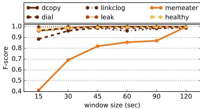
Fig. 3. The impact of window size on the per-class F-scores of the AdaBoost classifier. The F-score of memearer anomaly decreases significantly as window size get smaller.
