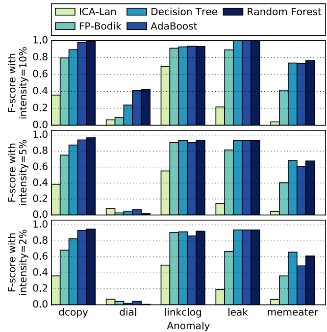
Fig. 11. Anomaly diagnosis statistics when the models are trained with anomaly intensities 20%, 50%, and 100%, and tested with intensities 2%, 5%, and 10%. Most anomaly signatures are detected when the intensity is lowered. In the dial anomaly, the intensity sets the utilization of the synthetic anomaly program, making it less impactful on the application performance and also harder to detect.
