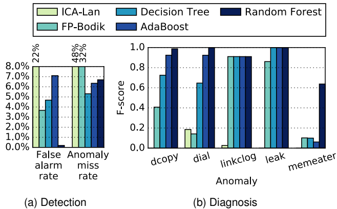
Fig. 12. Anomaly detection and diagnosis statistics when the models are trained with 4-node application runs and tested with 32-node runs. The results are very similar to those with unknown input configurations as the 32-node runs use input configurations that are not used for training.
