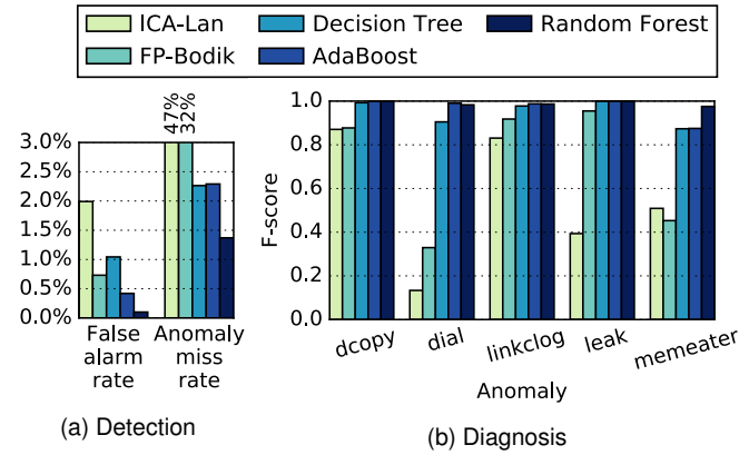
Fig. 7. Anomaly detection and diagnosis statistics of various classifiers using 5-fold stratified cross-validation. Random forest correctly identifies 98% of the anomalies while leading to only 0.08% false anomaly alarms.
