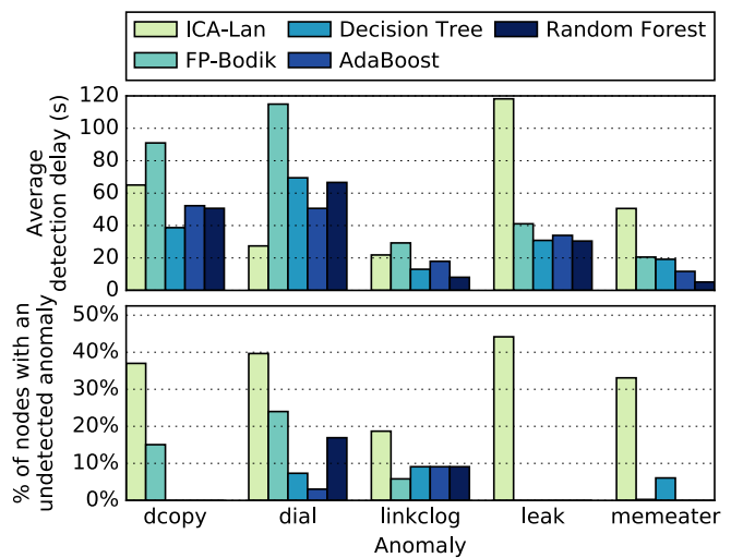
Fig. 13. Anomaly detection delay and percentage of nodes with undetected anomalies when anomalies start at a random time while the application is running.
