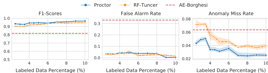
Fig. 3. Comparing the anomaly detection performance of Proctor with AE-Borghesi and RF-Tuncer in Eclipse data set. Proctor outperforms the baselines in F1-score and anomaly miss rate while maintaining a similar false alarm rate with RF-Tuncer.
