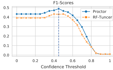
Fig. 6. Choosing a threshold that gives the highest F1-score by sweeping confidence thresholds.
